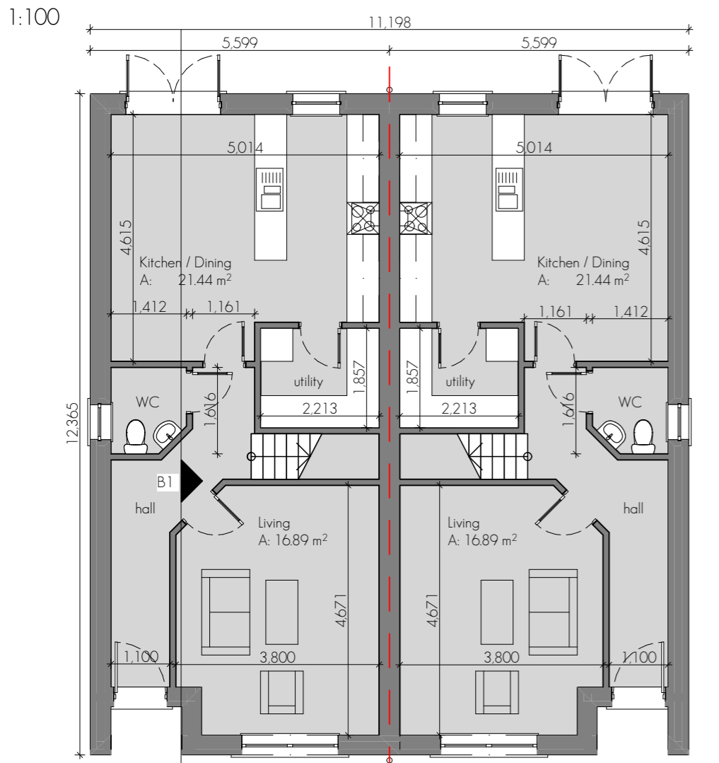
GROUND FLOOR B1/B1 1:100
