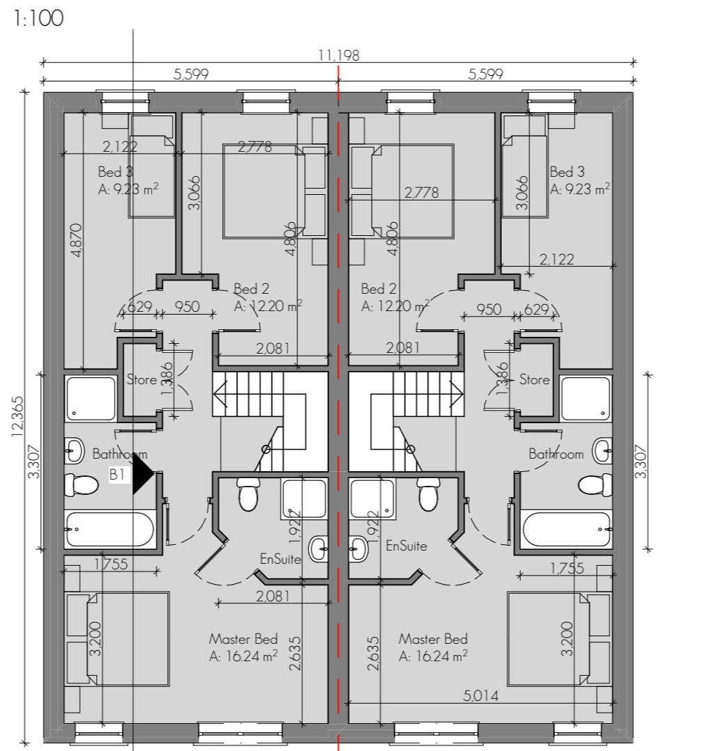
FIRST FLOOR B1/B1 1:100
